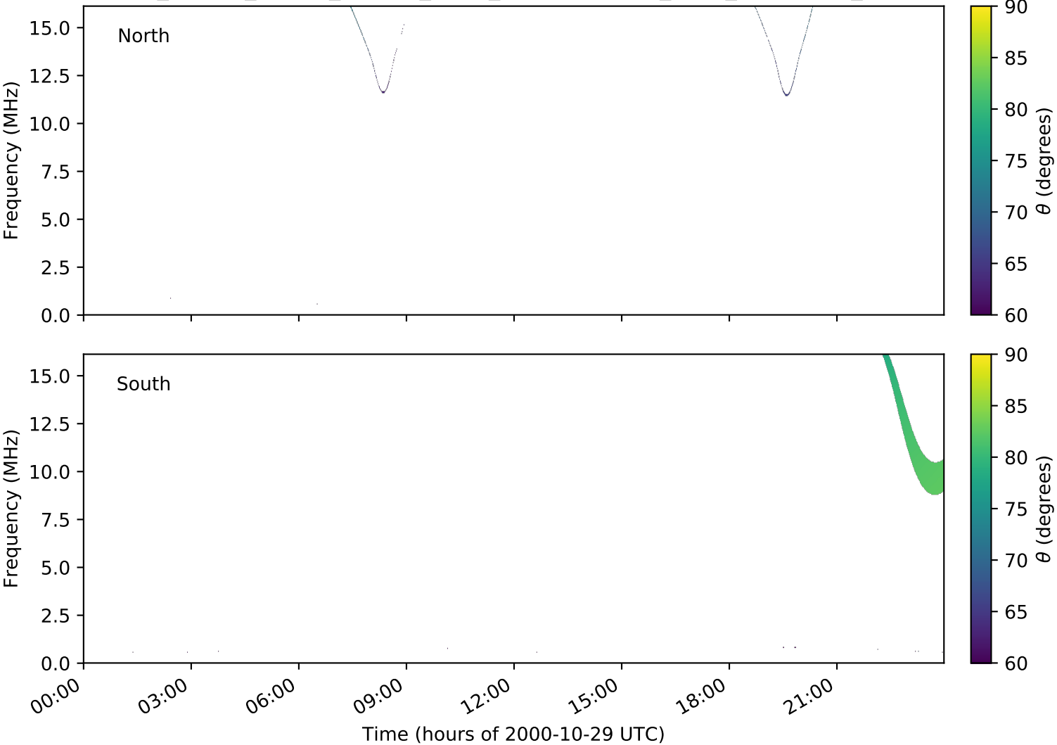
expres_cassini_jupiter_europa_isaac_lossc-wid1deg_3kev_20001029_v01.cdf
