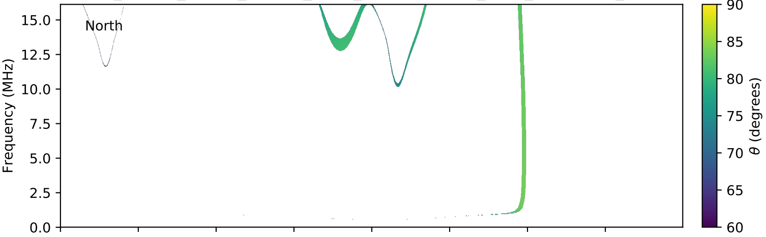
expres_cassini_jupiter_europa_isaac_lossc-wid1deg_3kev_20001026_v01.cdf
