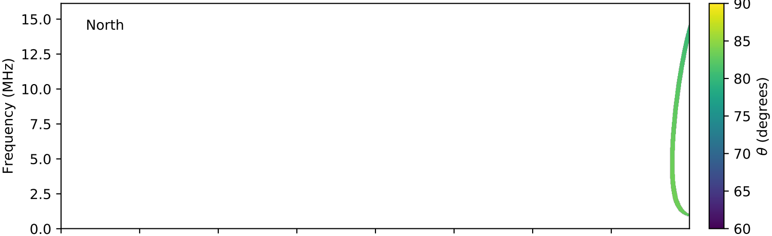
expres_cassini_jupiter_europa_isaac_lossc-wid1deg_3kev_20001024_v01.cdf
