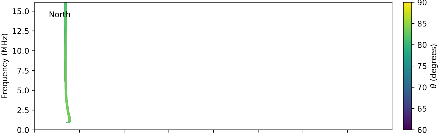
expres_cassini_jupiter_europa_isaac_lossc-wid1deg_3kev_20001023_v01.cdf
