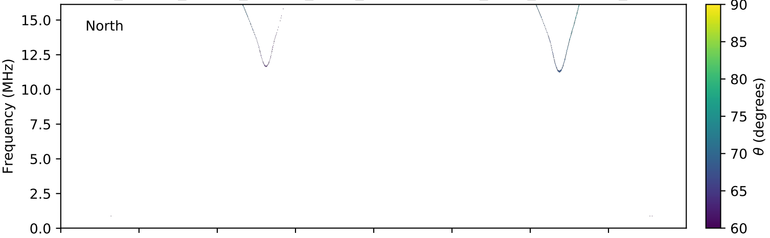
expres_cassini_jupiter_europa_isaac_lossc-wid1deg_3kev_20001022_v01.cdf
