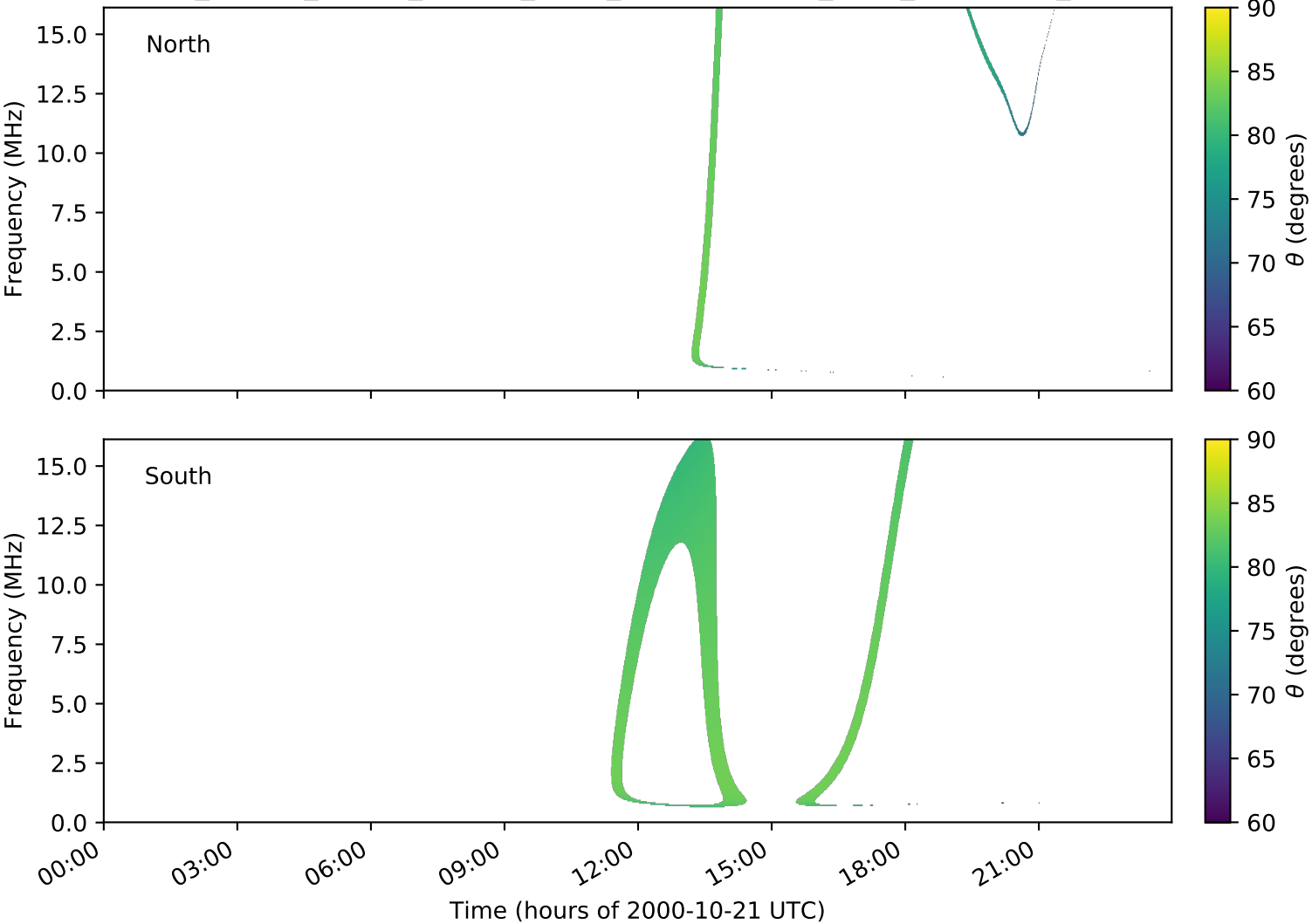
expres_cassini_jupiter_europa_isaac_lossc-wid1deg_3kev_20001021_v01.cdf
