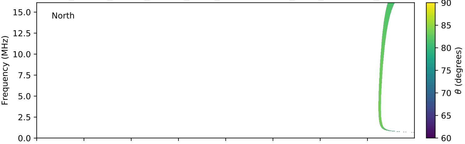
expres_cassini_jupiter_europa_isaac_lossc-wid1deg_3kev_20001017_v01.cdf
