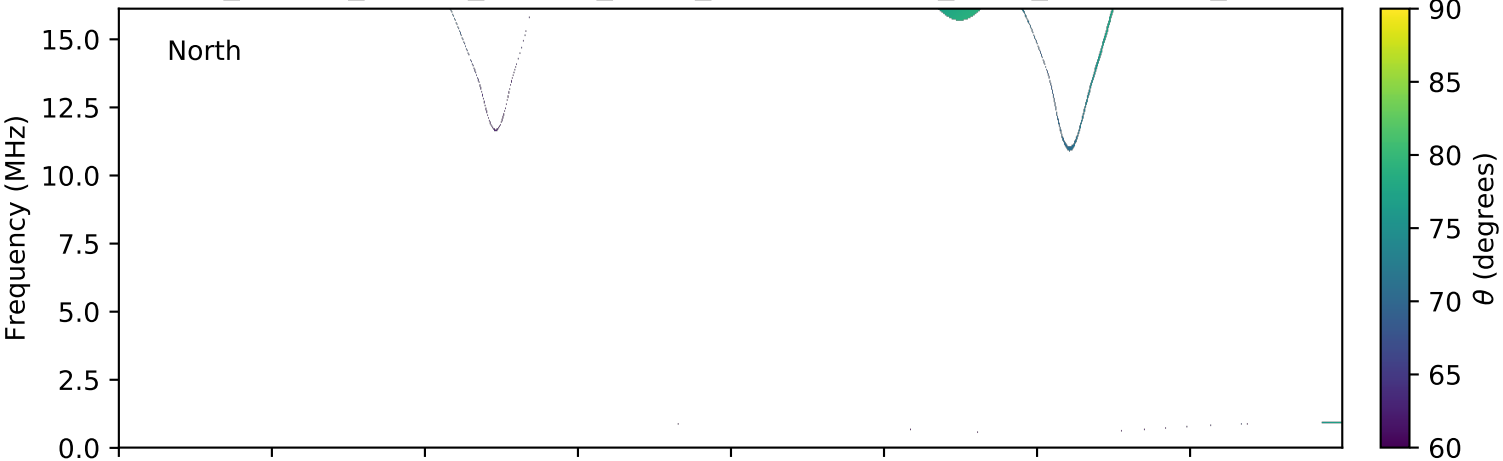
expres_cassini_jupiter_europa_isaac_lossc-wid1deg_3kev_20001015_v01.cdf
