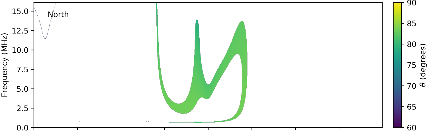
expres_cassini_jupiter_europa_isaac_lossc-wid1deg_3kev_20001012_v01.cdf
