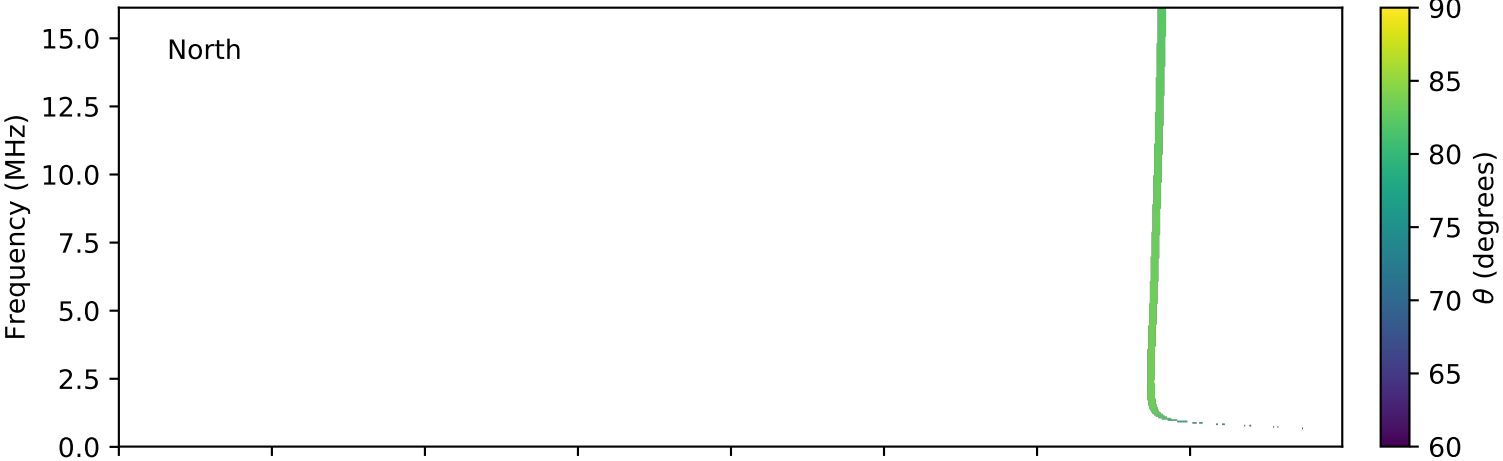
expres_cassini_jupiter_europa_isaac_lossc-wid1deg_3kev_20001010_v01.cdf
