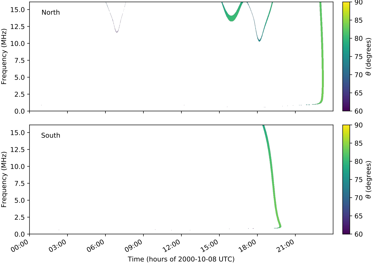
expres_cassini_jupiter_europa_isaac_lossc-wid1deg_3kev_20001008_v01.cdf
