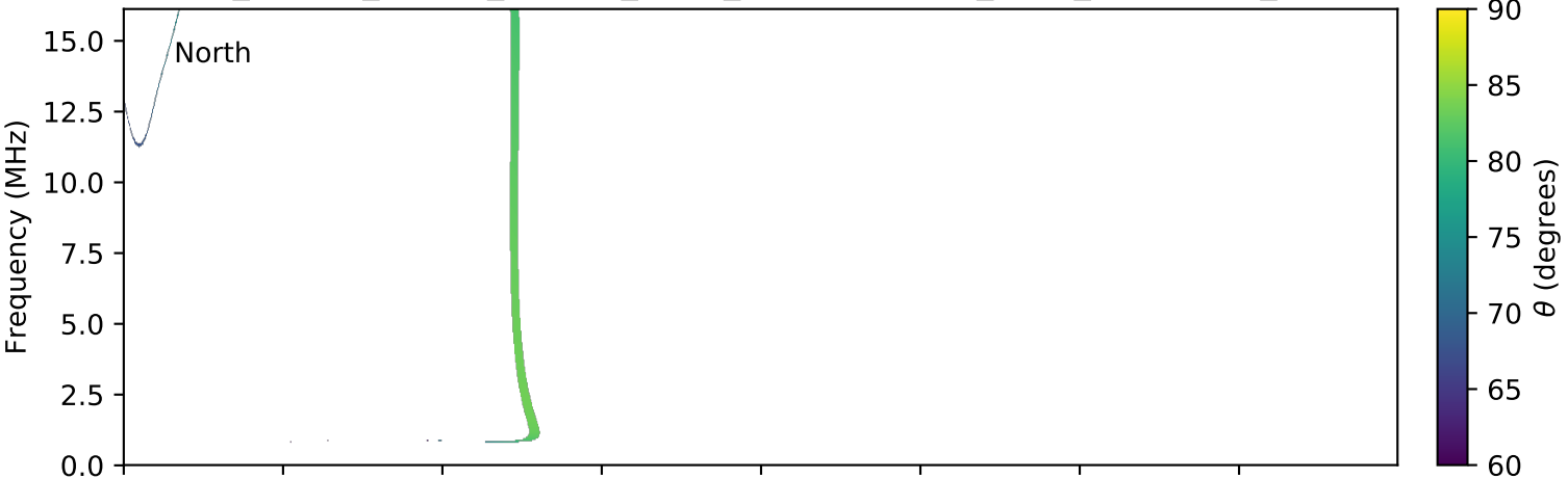
expres_cassini_jupiter_europa_isaac_lossc-wid1deg_3kev_20001005_v01.cdf
