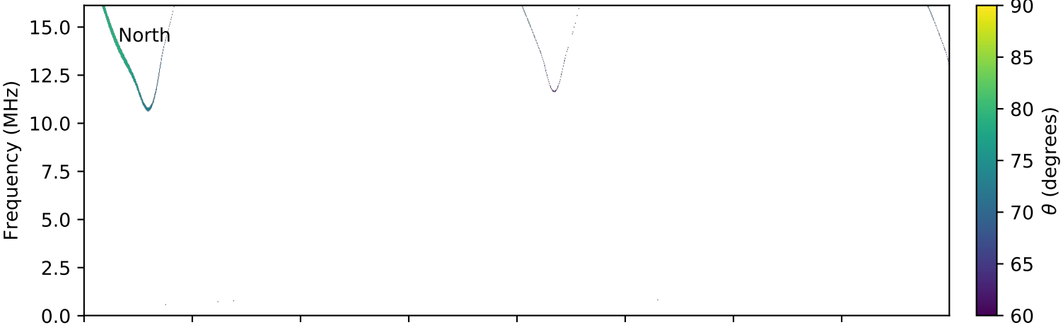
expres_cassini_jupiter_europa_isaac_lossc-wid1deg_3kev_20001004_v01.cdf
