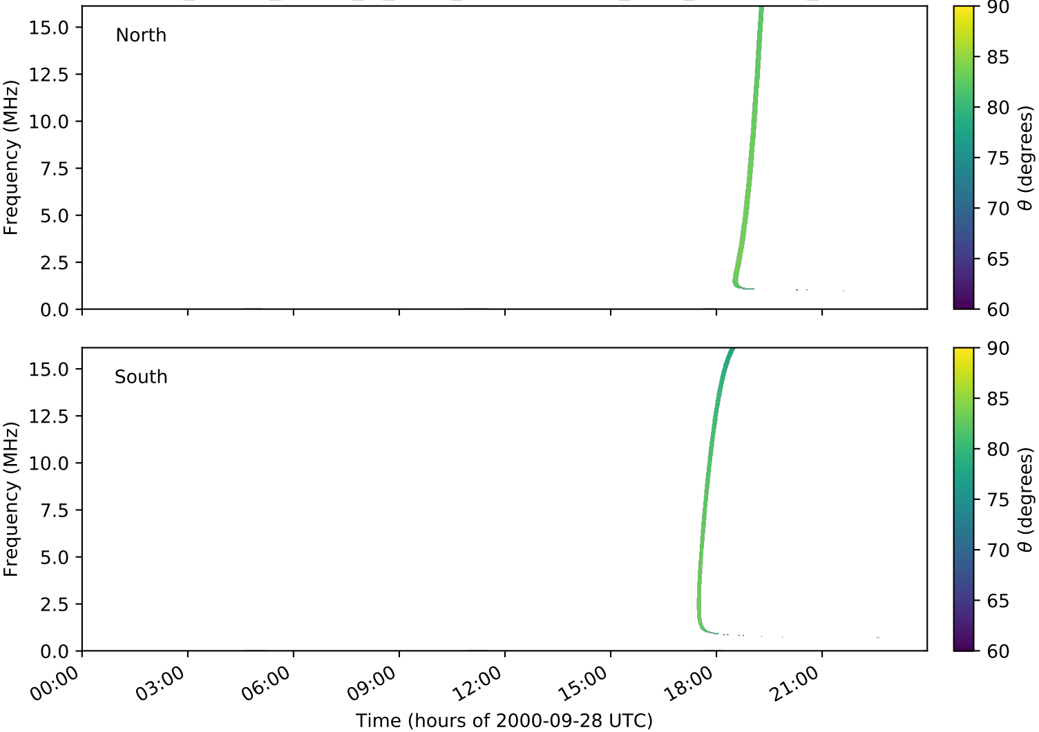
expres_cassini_jupiter_io_isaac_lossc-wid1deg_3kev_20000928_v01.cdf
