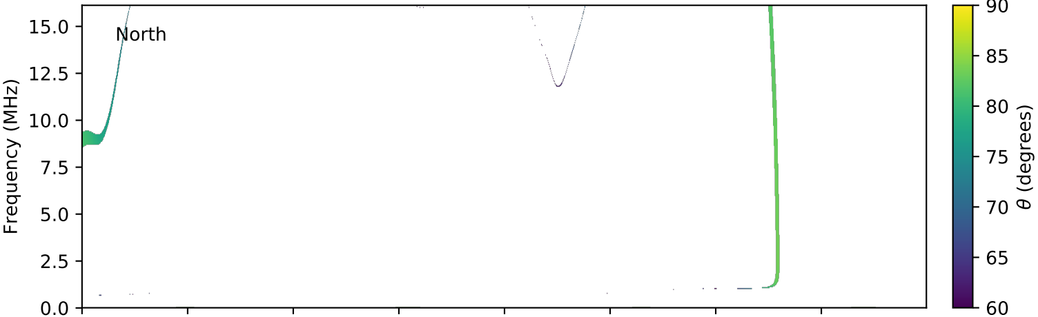
expres_cassini_jupiter_io_isaac_lossc-wid1deg_3kev_20000927_v01.cdf
