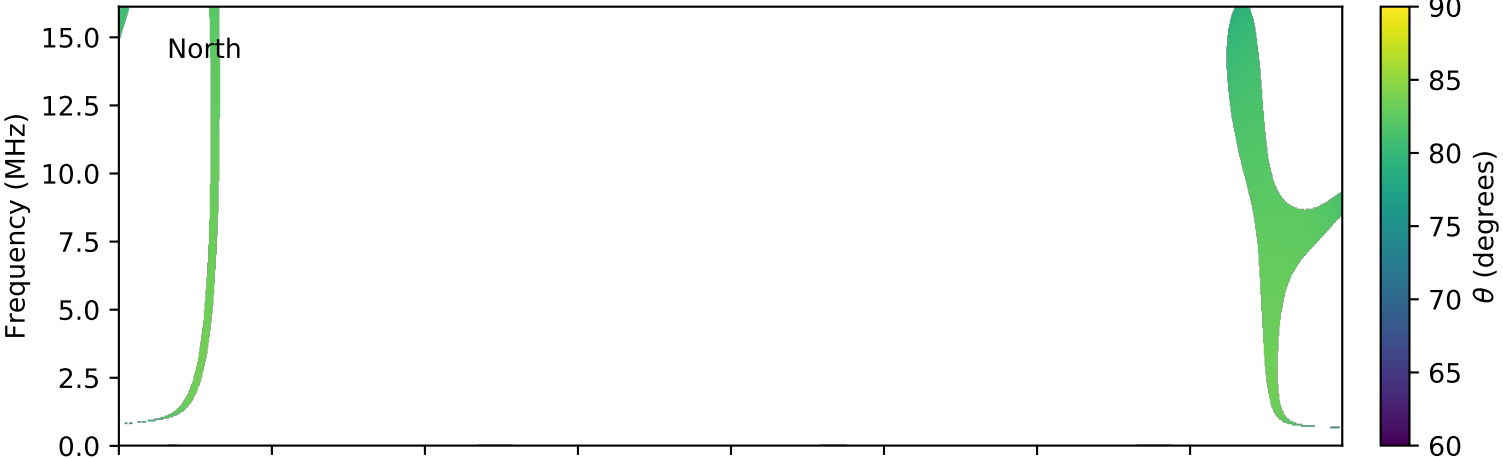
expres_cassini_jupiter_io_isaac_lossc-wid1deg_3kev_20000926_v01.cdf
