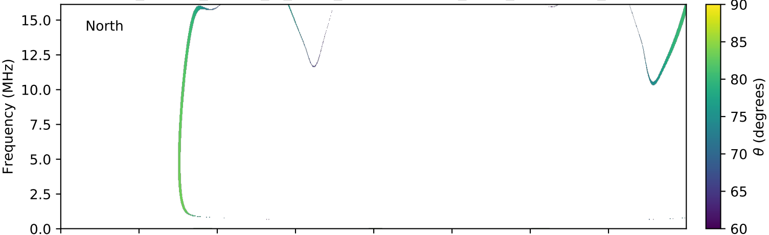
expres_cassini_jupiter_io_isaac_lossc-wid1deg_3kev_20000925_v01.cdf
