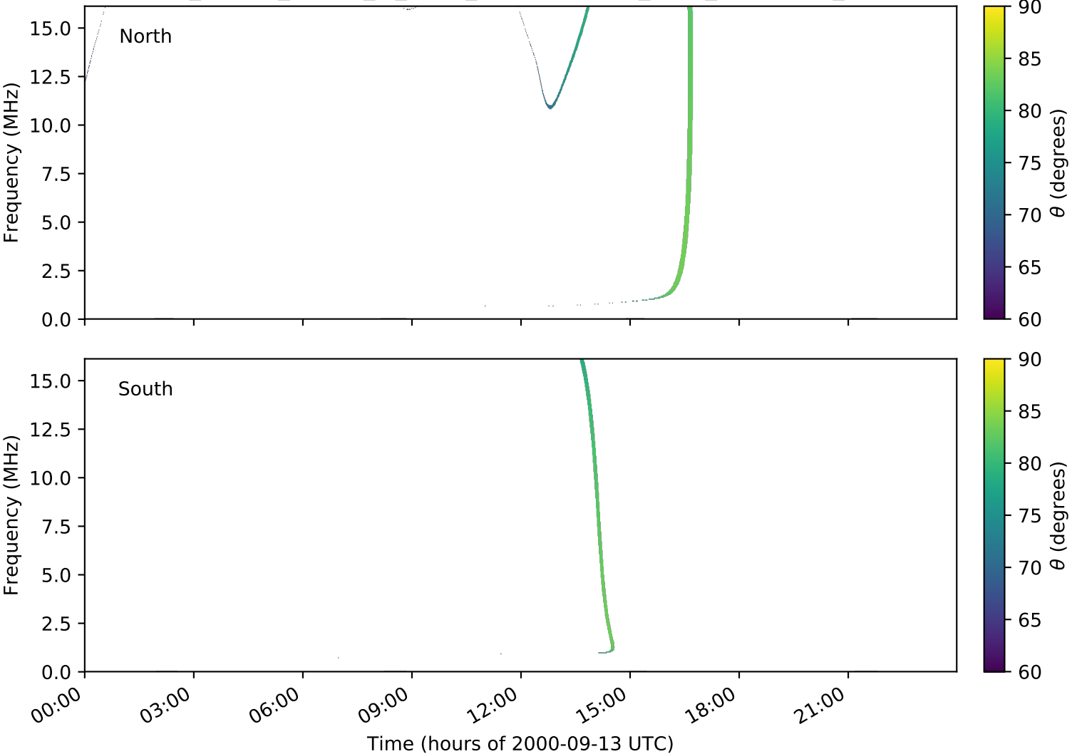
expres_cassini_jupiter_io_isaac_lossc-wid1deg_3kev_20000913_v01.cdf
