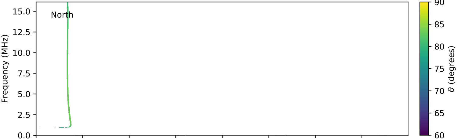
expres_cassini_jupiter_io_isaac_lossc-wid1deg_3kev_20000910_v01.cdf
