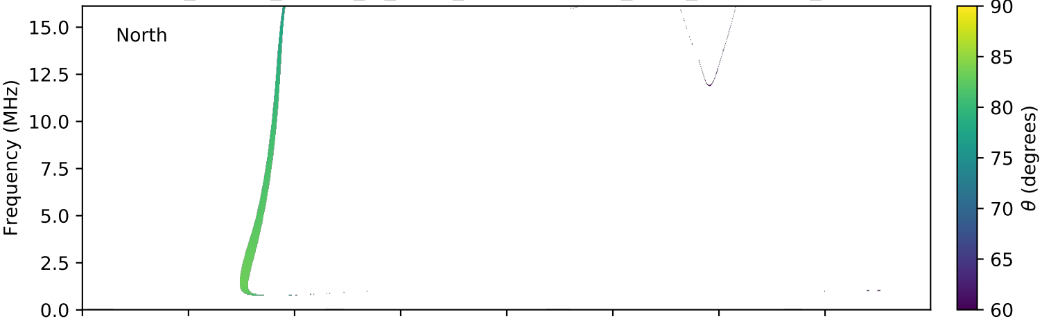
expres_cassini_jupiter_io_isaac_lossc-wid1deg_3kev_20000902_v01.cdf
