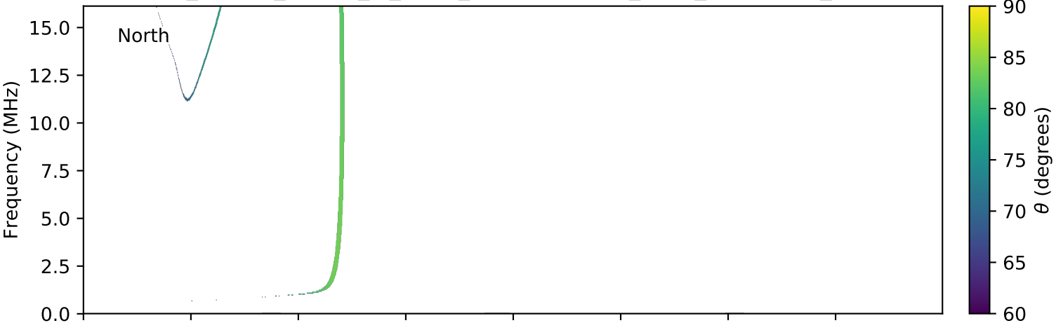
expres_cassini_jupiter_io_isaac_lossc-wid1deg_3kev_20000901_v01.cdf
