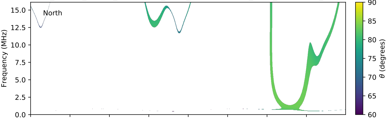
expres_cassini_jupiter_ganymede_isaac_lossc-wid1deg_3kev_20000930_v01.cdf
