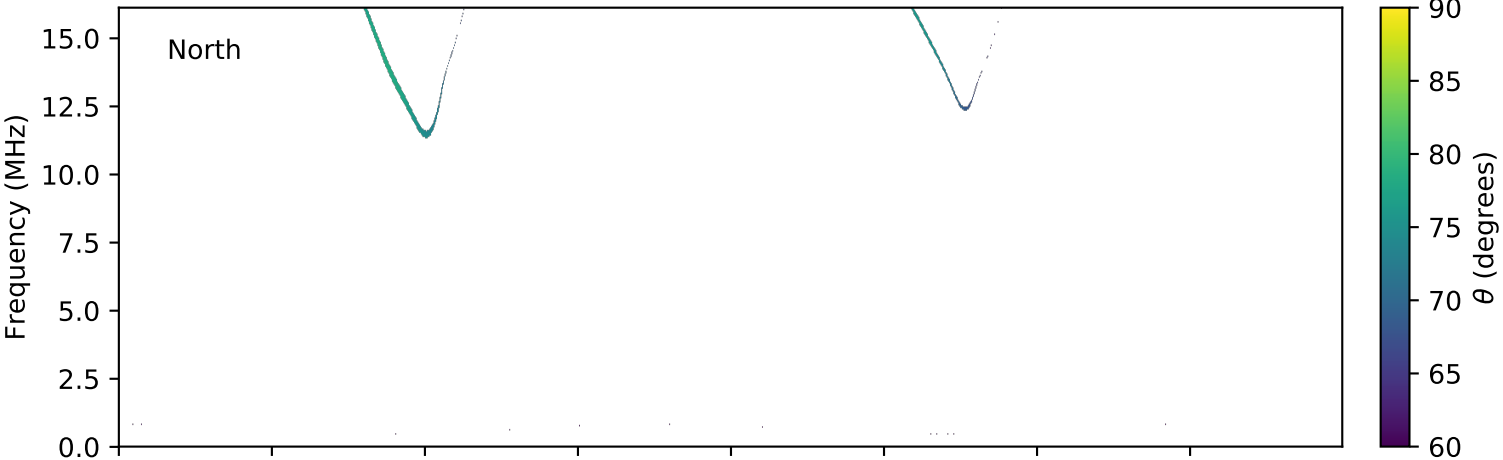
expres_cassini_jupiter_ganymede_isaac_lossc-wid1deg_3kev_20000921_v01.cdf
