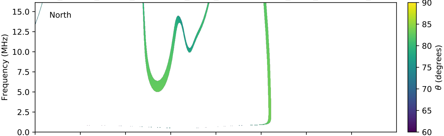
expres_cassini_jupiter_ganymede_isaac_lossc-wid1deg_3kev_20000916_v01.cdf
