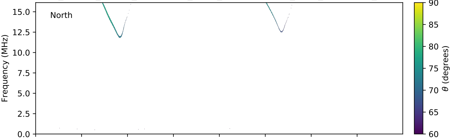
expres_cassini_jupiter_ganymede_isaac_lossc-wid1deg_3kev_20000914_v01.cdf
