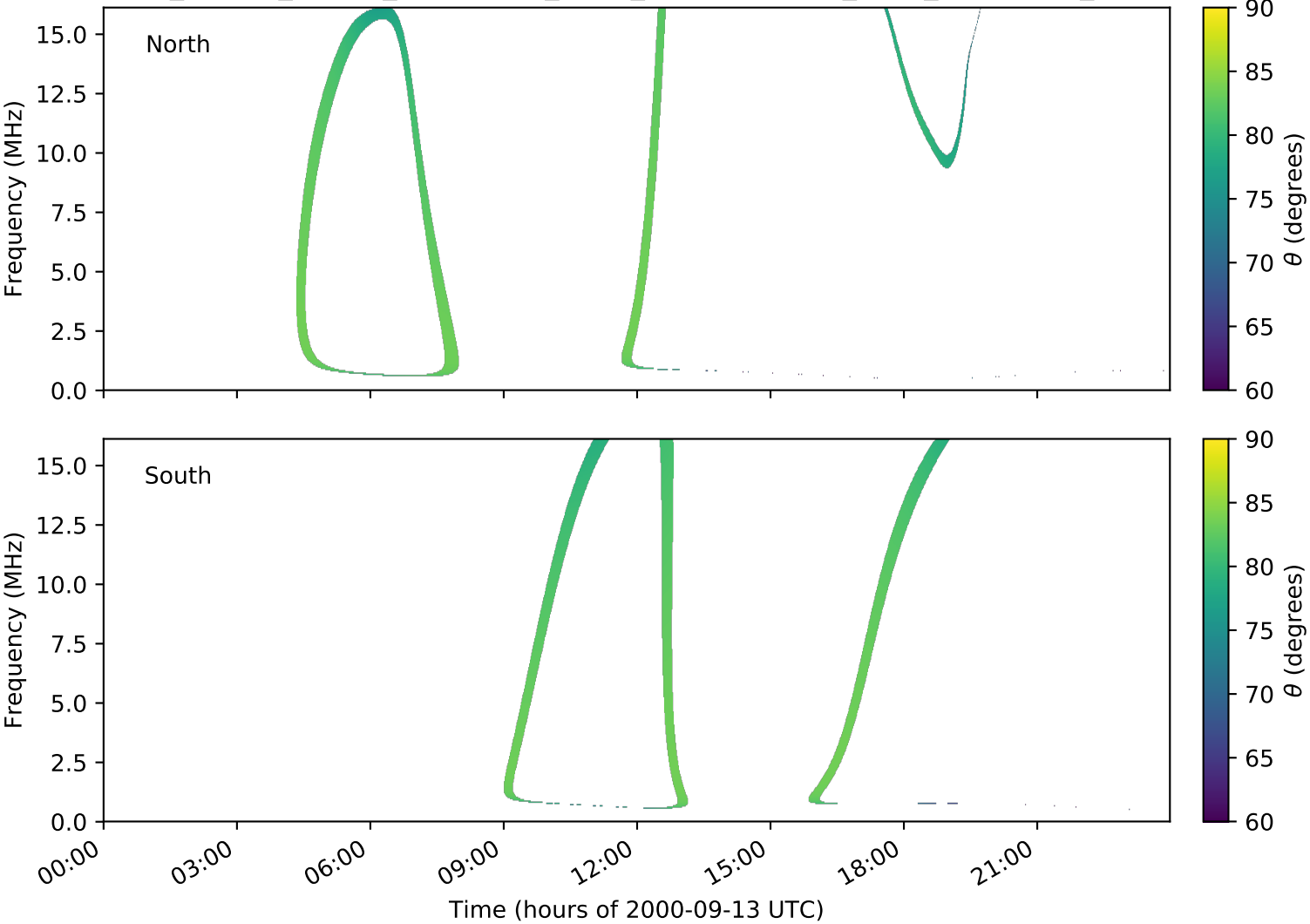
expres_cassini_jupiter_ganymede_isaac_lossc-wid1deg_3kev_20000913_v01.cdf
