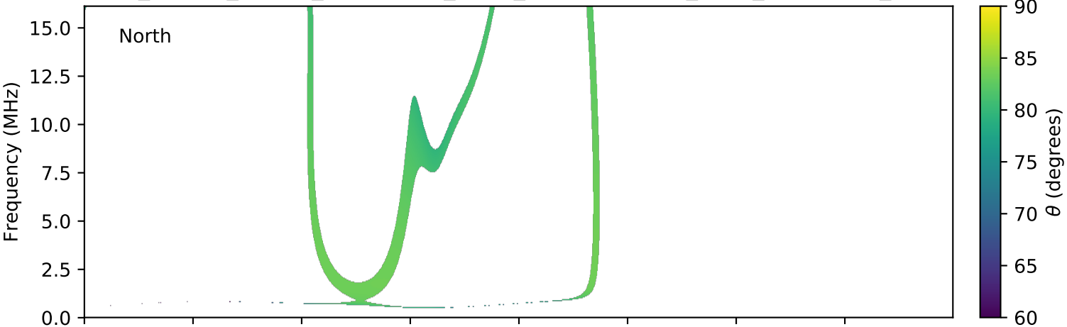
expres_cassini_jupiter_ganymede_isaac_lossc-wid1deg_3kev_20000909_v01.cdf
