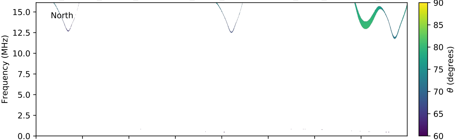
expres_cassini_jupiter_ganymede_isaac_lossc-wid1deg_3kev_20000908_v01.cdf
