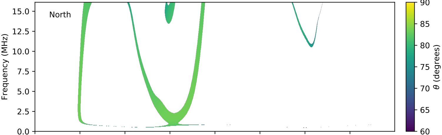
expres_cassini_jupiter_ganymede_isaac_lossc-wid1deg_3kev_20000906_v01.cdf
