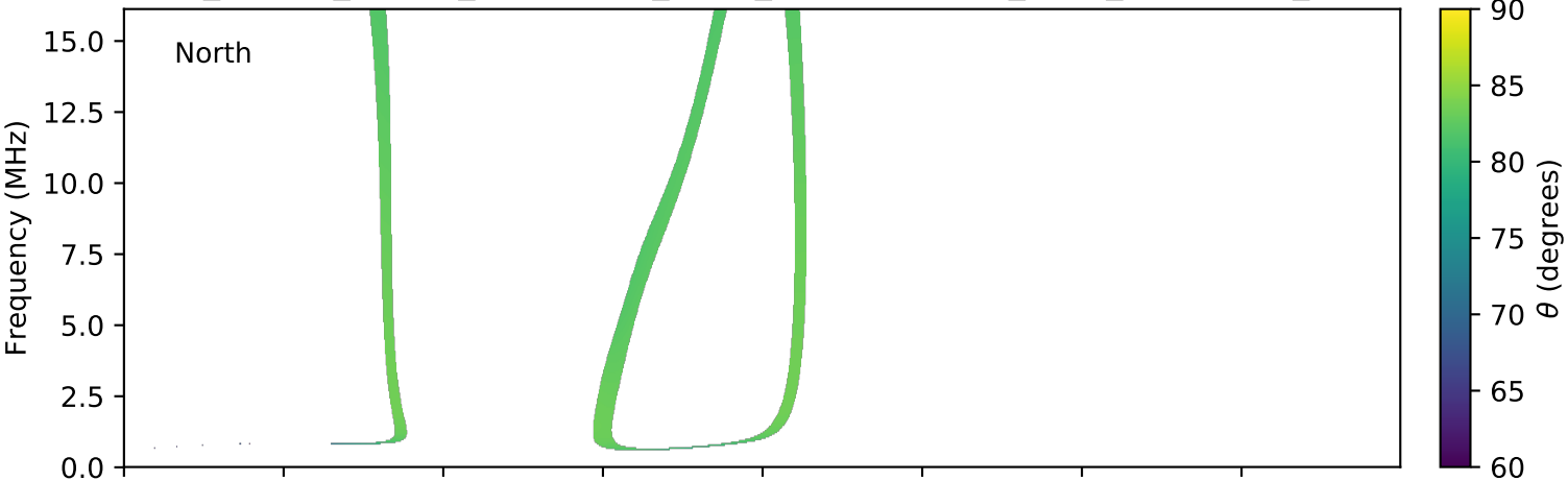
expres_cassini_jupiter_ganymede_isaac_lossc-wid1deg_3kev_20000902_v01.cdf
