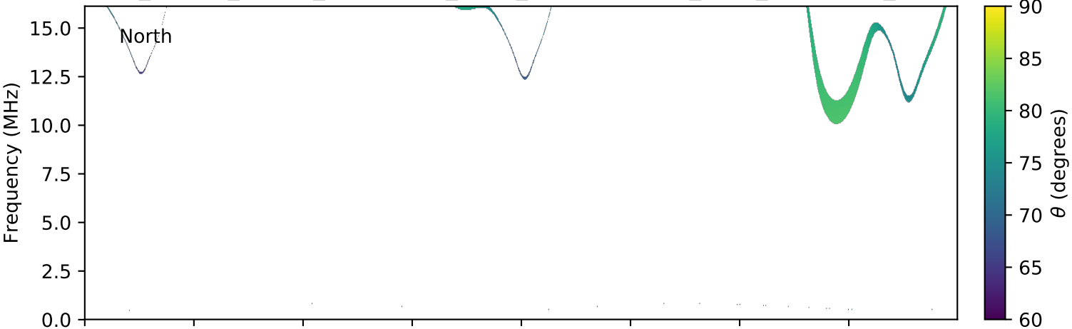
expres_cassini_jupiter_ganymede_isaac_lossc-wid1deg_3kev_20000901_v01.cdf
