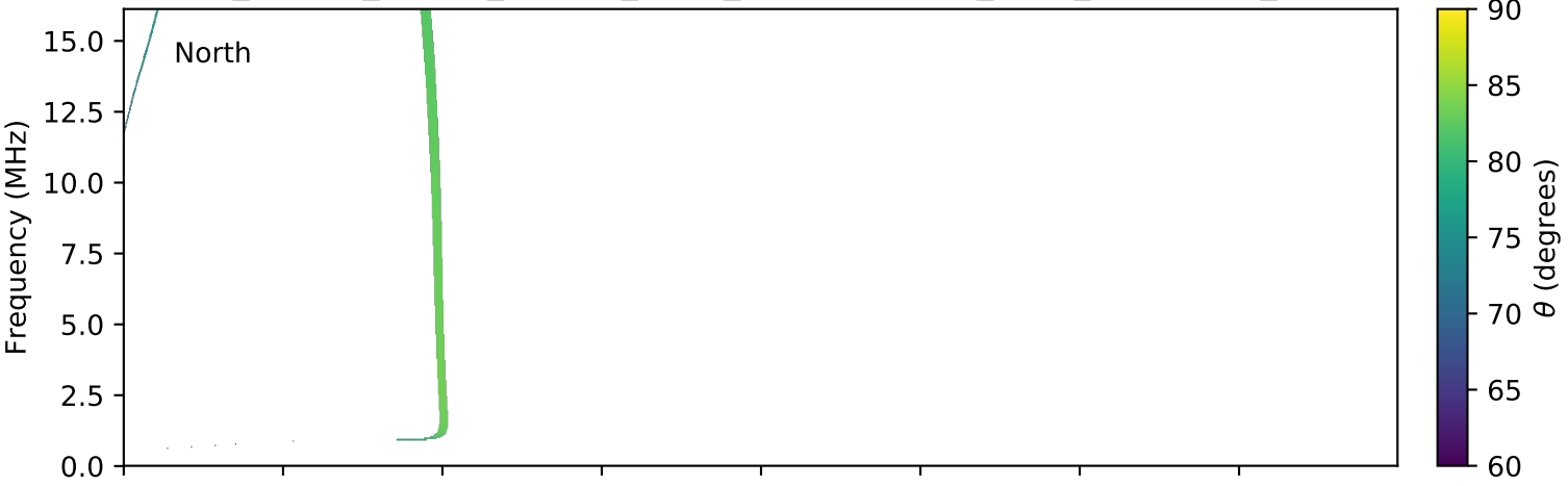
expres_cassini_jupiter_europa_isaac_lossc-wid1deg_3kev_20000928_v01.cdf
