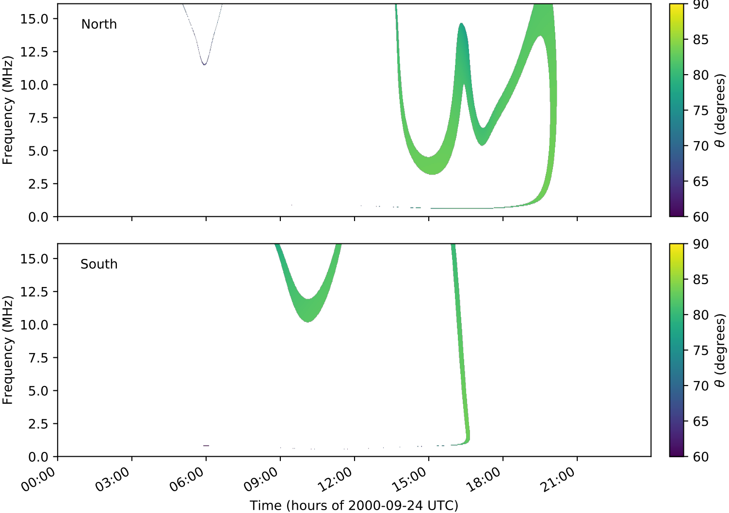
expres_cassini_jupiter_europa_isaac_lossc-wid1deg_3kev_20000924_v01.cdf
