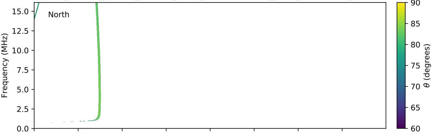
expres_cassini_jupiter_europa_isaac_lossc-wid1deg_3kev_20000921_v01.cdf
