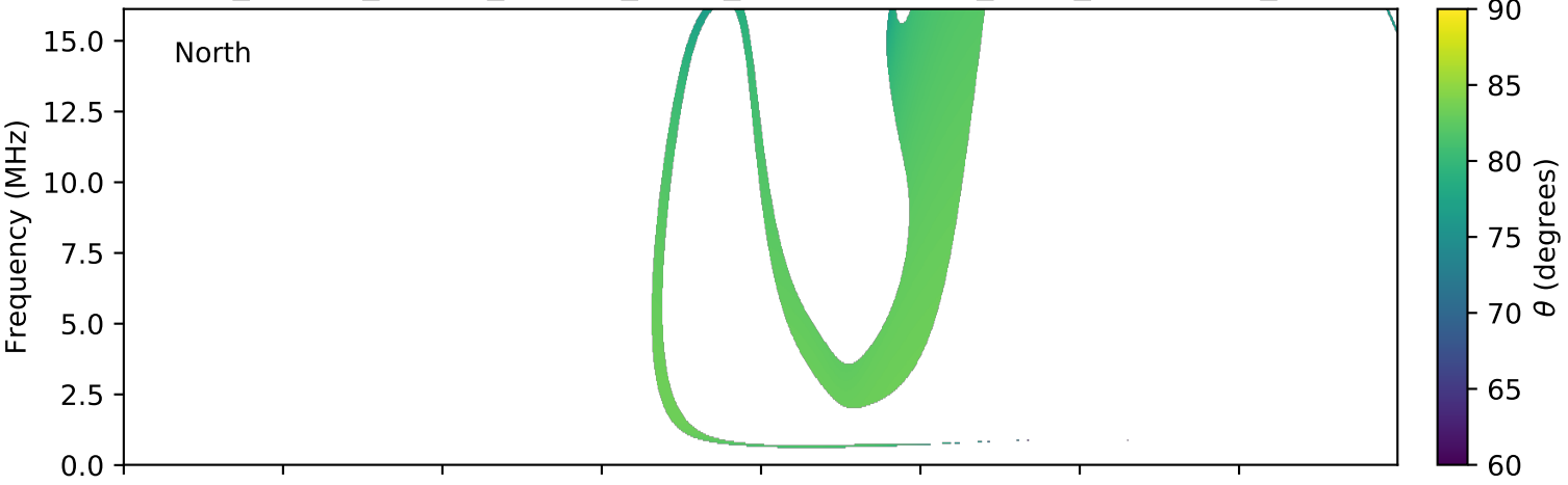
expres_cassini_jupiter_europa_isaac_lossc-wid1deg_3kev_20000919_v01.cdf
