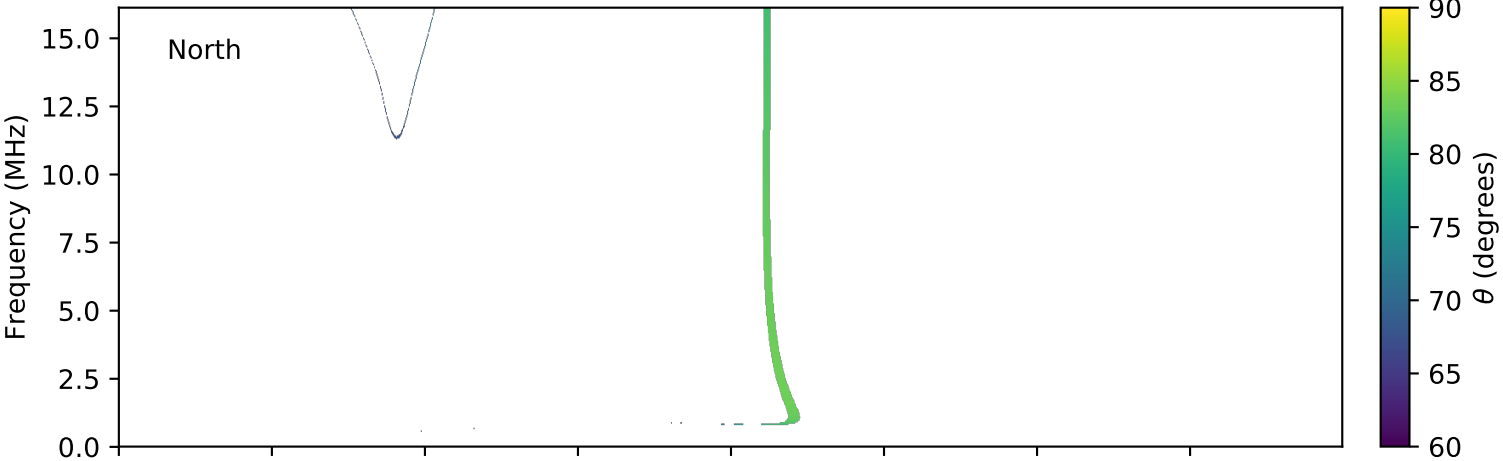
expres_cassini_jupiter_europa_isaac_lossc-wid1deg_3kev_20000917_v01.cdf
