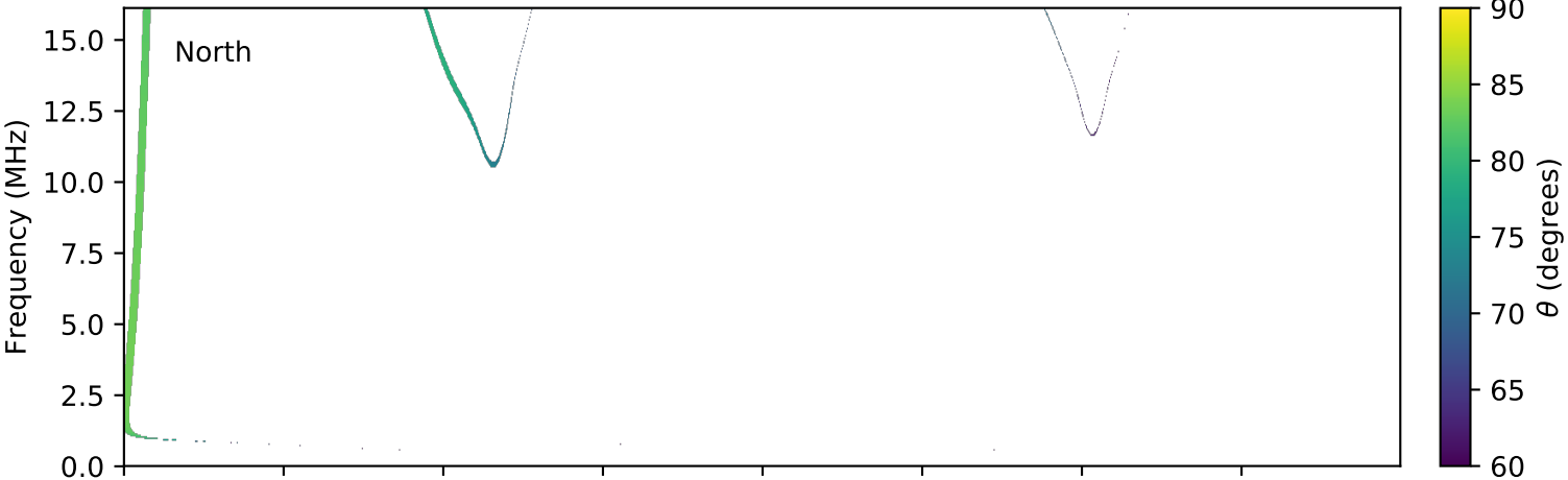
expres_cassini_jupiter_europa_isaac_lossc-wid1deg_3kev_20000916_v01.cdf
