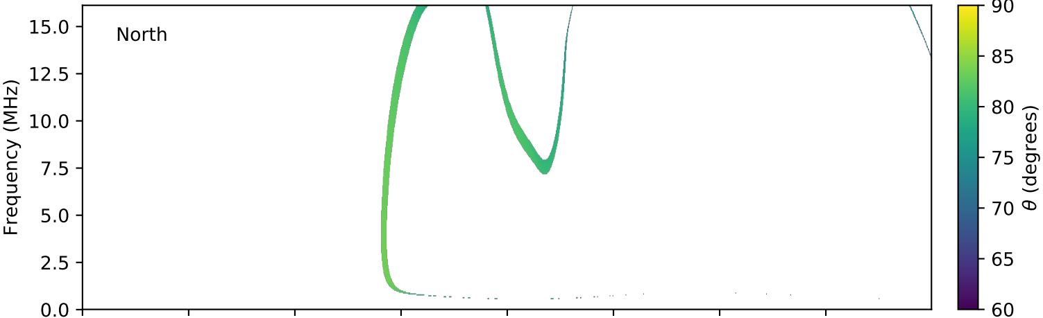
expres_cassini_jupiter_europa_isaac_lossc-wid1deg_3kev_20000912_v01.cdf
