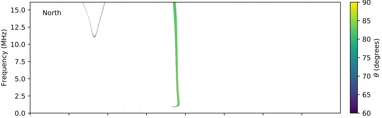
expres_cassini_jupiter_europa_isaac_lossc-wid1deg_3kev_20000910_v01.cdf
