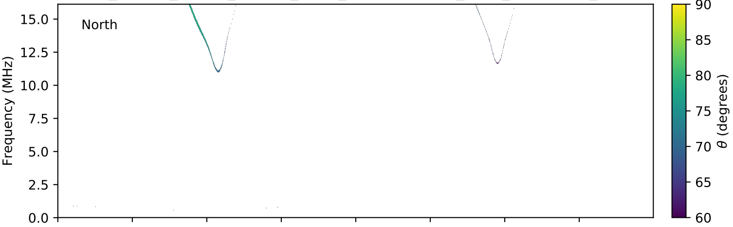
expres_cassini_jupiter_europa_isaac_lossc-wid1deg_3kev_20000909_v01.cdf
