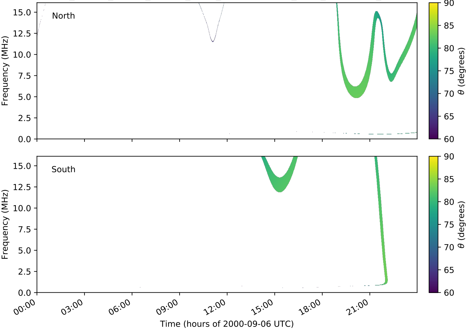
expres_cassini_jupiter_europa_isaac_lossc-wid1deg_3kev_20000906_v01.cdf
