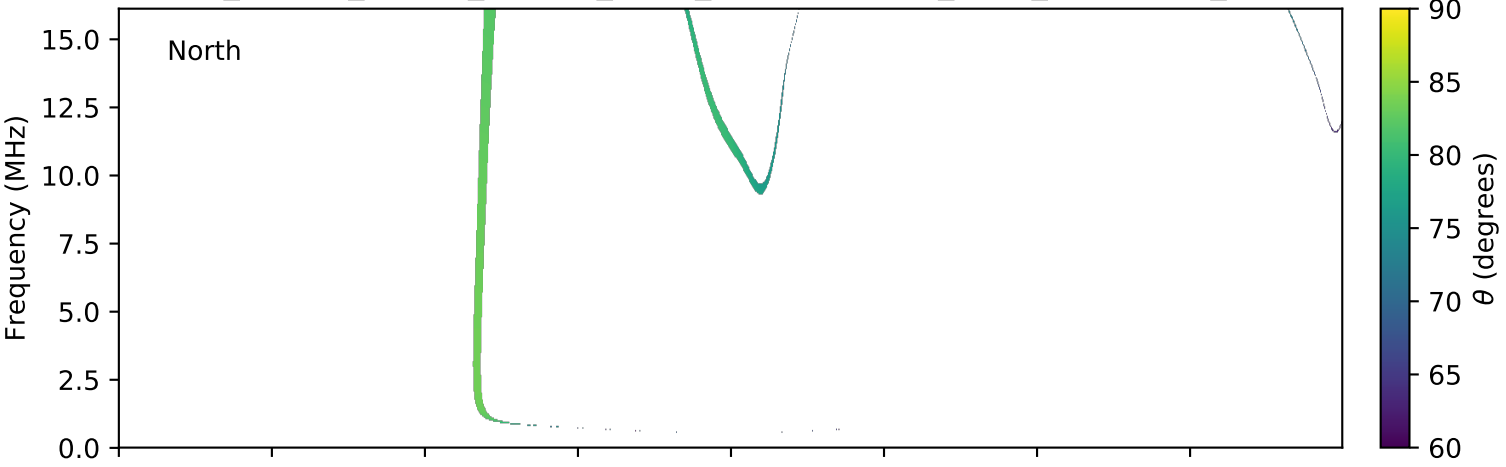
expres_cassini_jupiter_europa_isaac_lossc-wid1deg_3kev_20000905_v01.cdf
