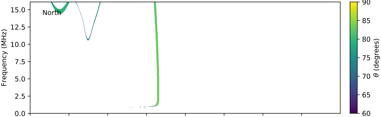
expres_cassini_jupiter_europa_isaac_lossc-wid1deg_3kev_20000903_v01.cdf
