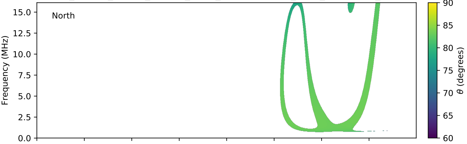
expres_cassini_jupiter_europa_isaac_lossc-wid1deg_3kev_20000901_v01.cdf
