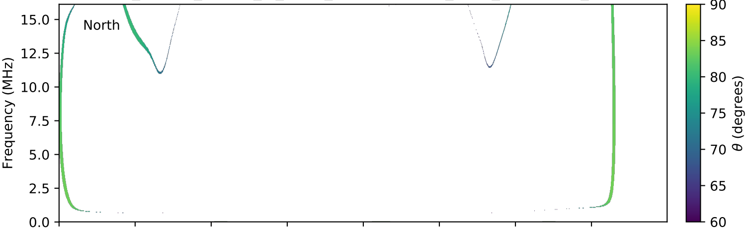
expres_cassini_jupiter_io_isaac_lossc-wid1deg_3kev_20000819_v01.cdf
