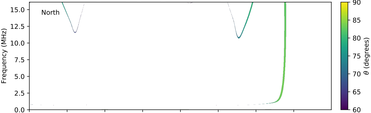
expres_cassini_jupiter_io_isaac_lossc-wid1deg_3kev_20000812_v01.cdf
