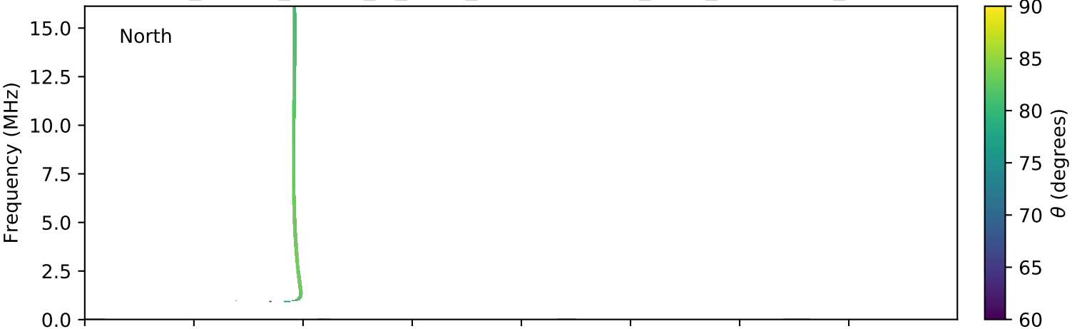
expres_cassini_jupiter_io_isaac_lossc-wid1deg_3kev_20000809_v01.cdf
