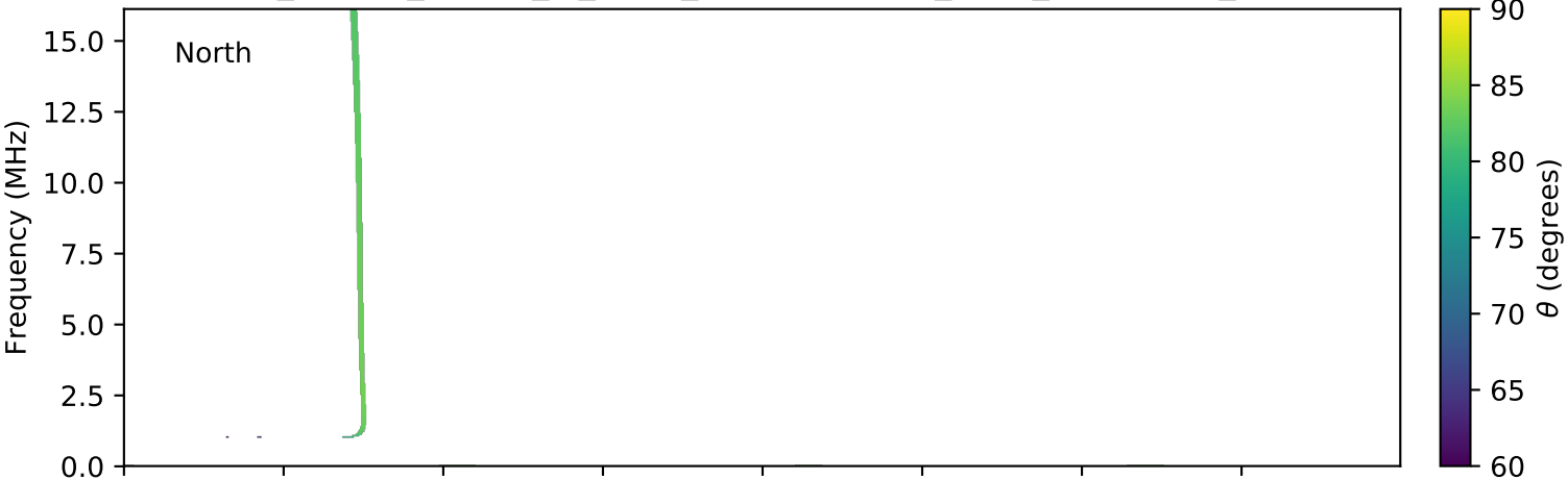
expres_cassini_jupiter_io_isaac_lossc-wid1deg_3kev_20000802_v01.cdf
