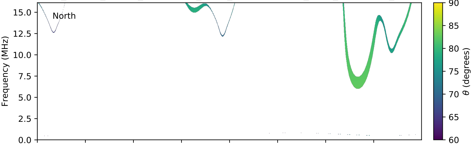
expres_cassini_jupiter_ganymede_isaac_lossc-wid1deg_3kev_20000825_v01.cdf
