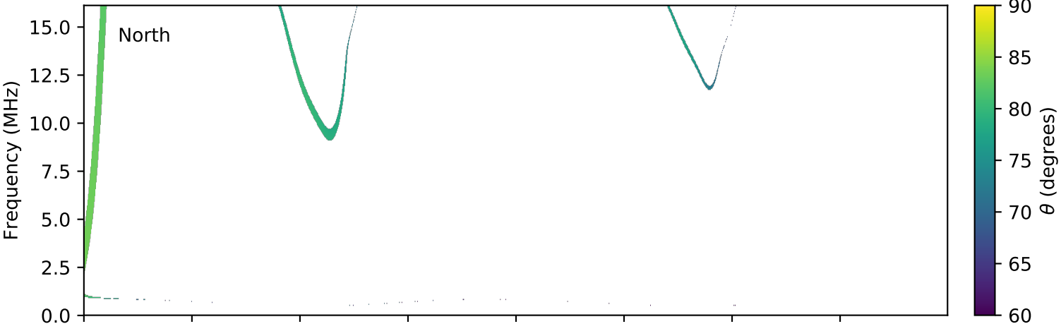
expres_cassini_jupiter_ganymede_isaac_lossc-wid1deg_3kev_20000823_v01.cdf
